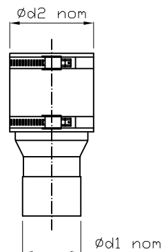
AUMENTO \phi 63/80 mm CON MANICOTTO IN IDRORAD ADAPTER KIT \phi 63/80 mm WITH COUPLING IN IDRORAD
